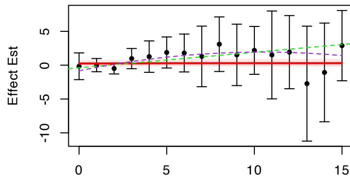
TEAD3: rs112518545
