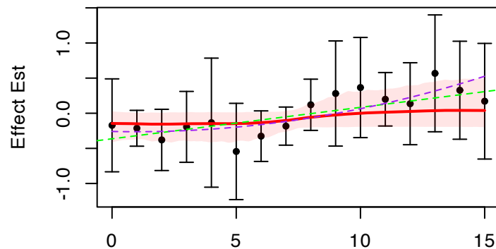
PLAUR: rs3786953
